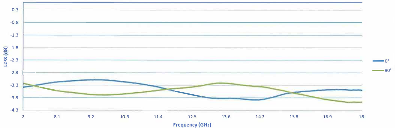
Insertion Loss
