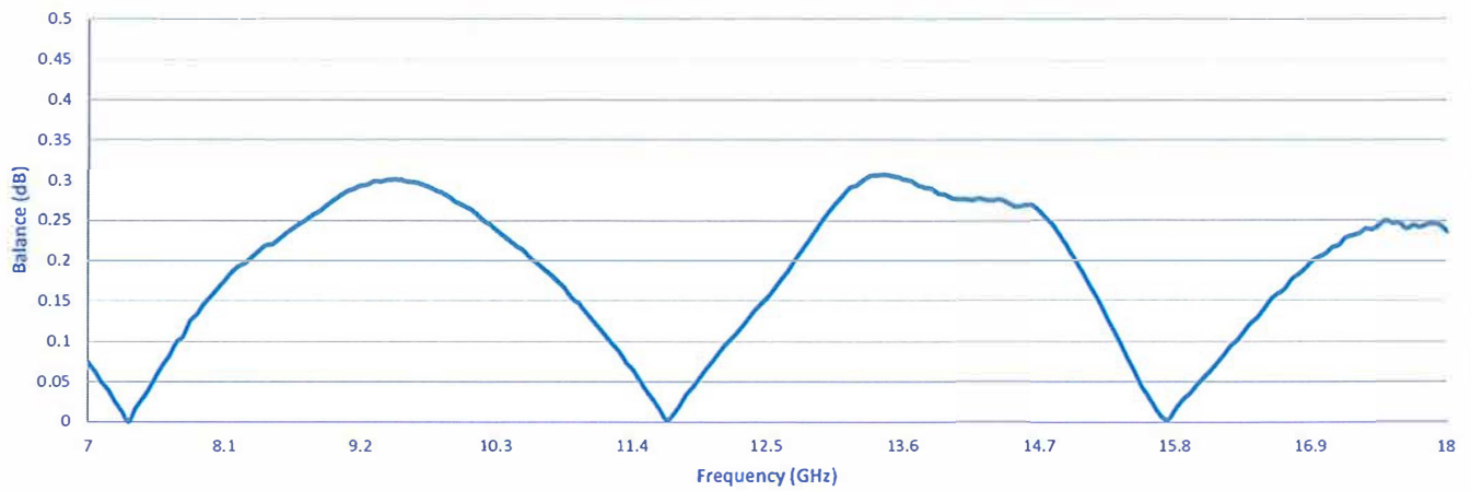
Amplitude Balance
