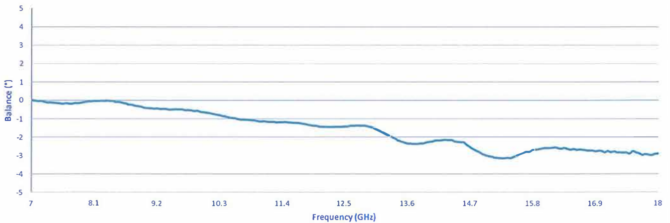
Phase Balance
