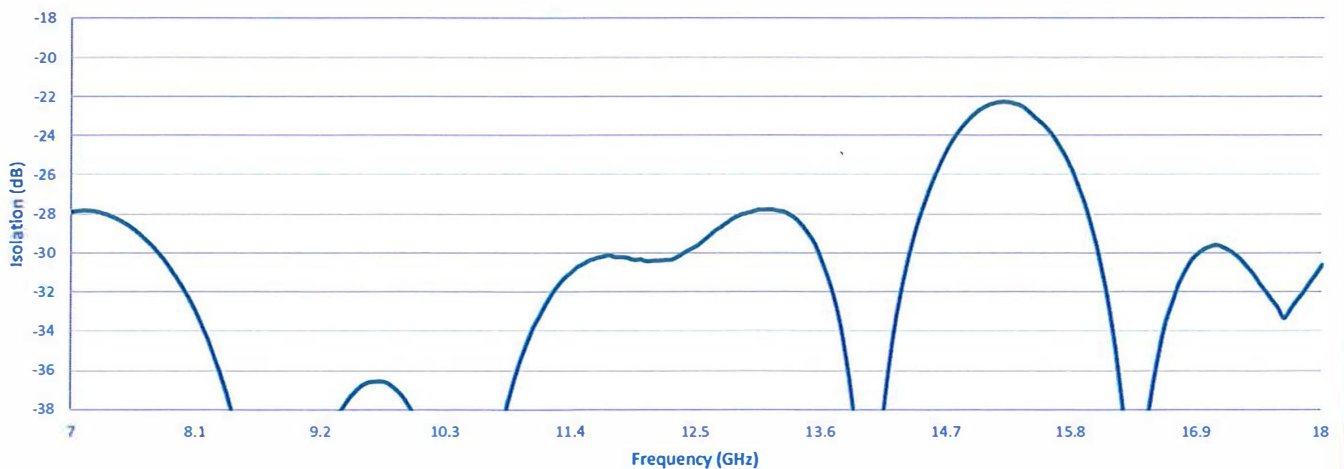
Isolation
