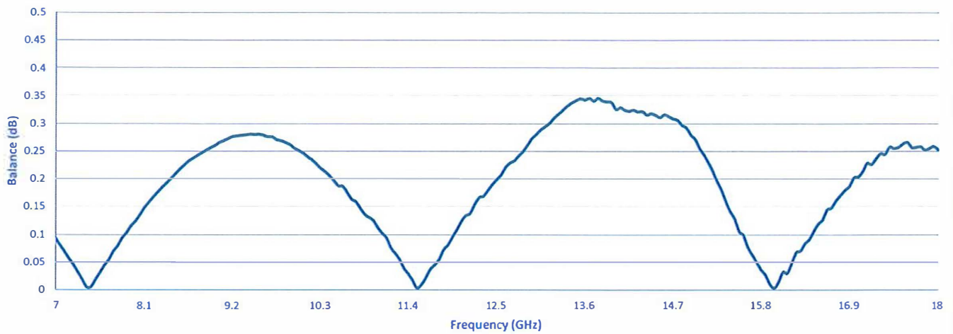
Amplitude Balance
