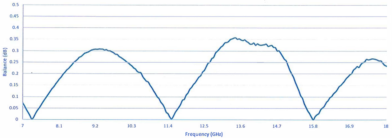
Amplitude Balance
