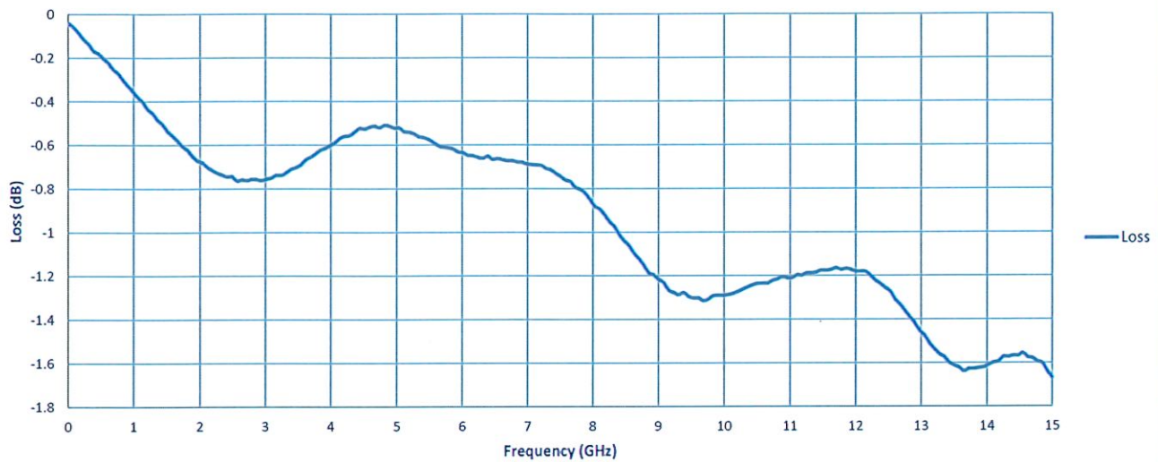
Insertion Loss
