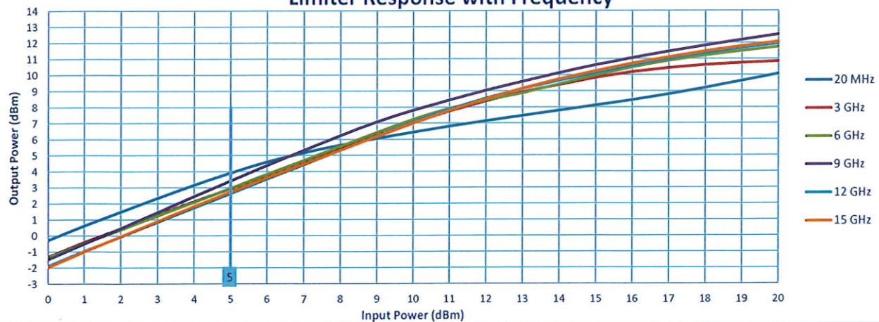
Limiter Response with Frequency
