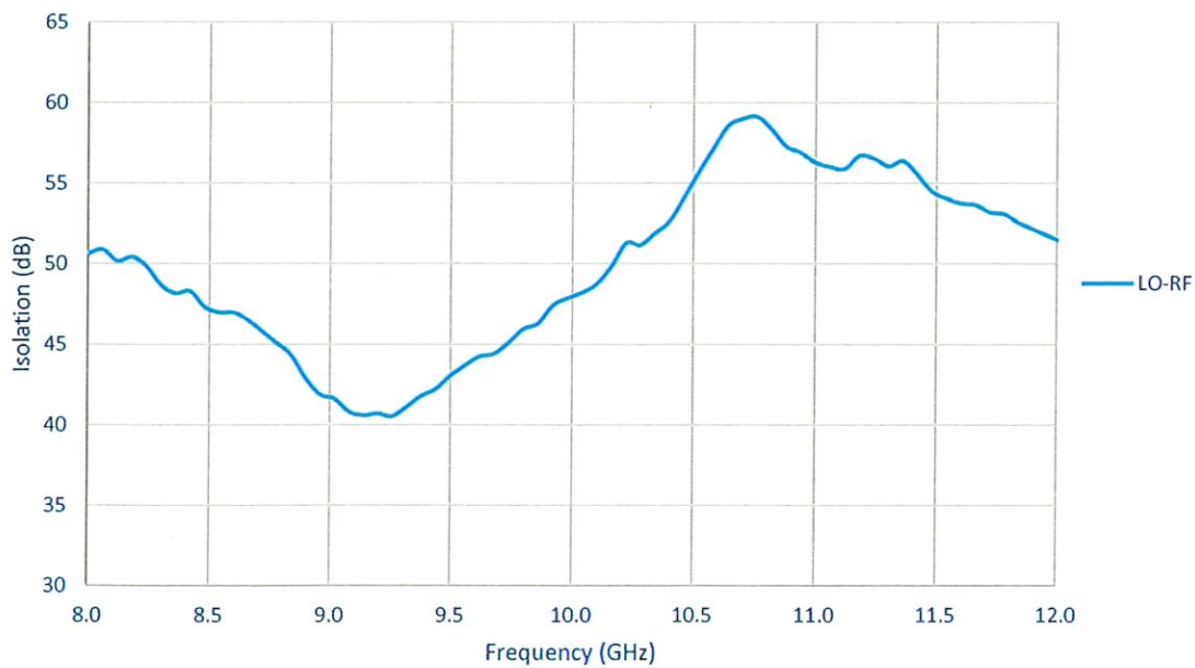
LO-RF Isolation
