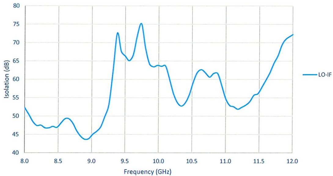
LO-IF Isolation
