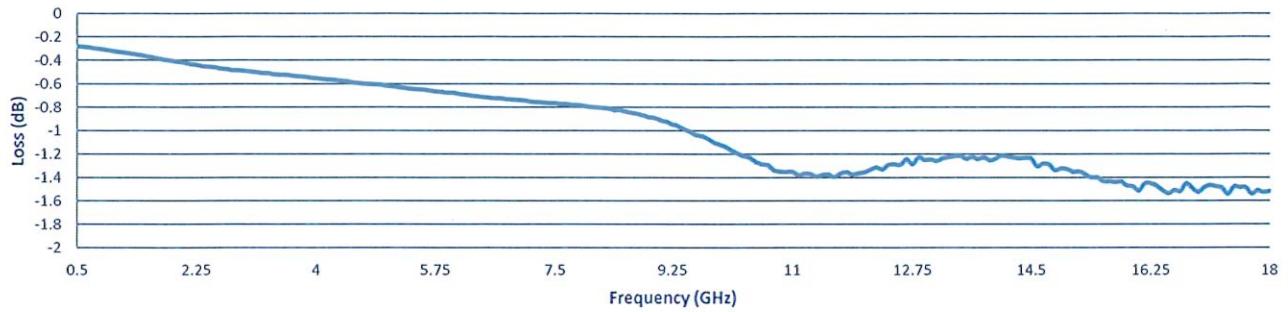
Insertion Loss @ -20 dB
