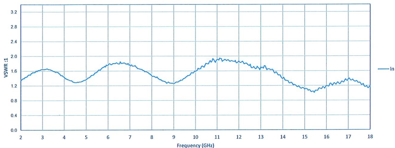
VSWR In
