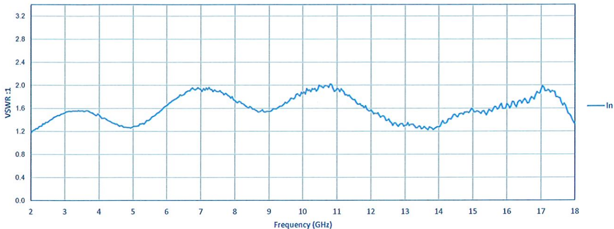
VSWR In
