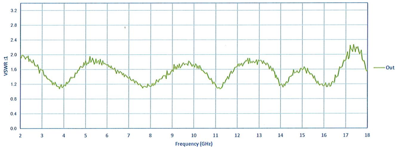
VSWR Out
