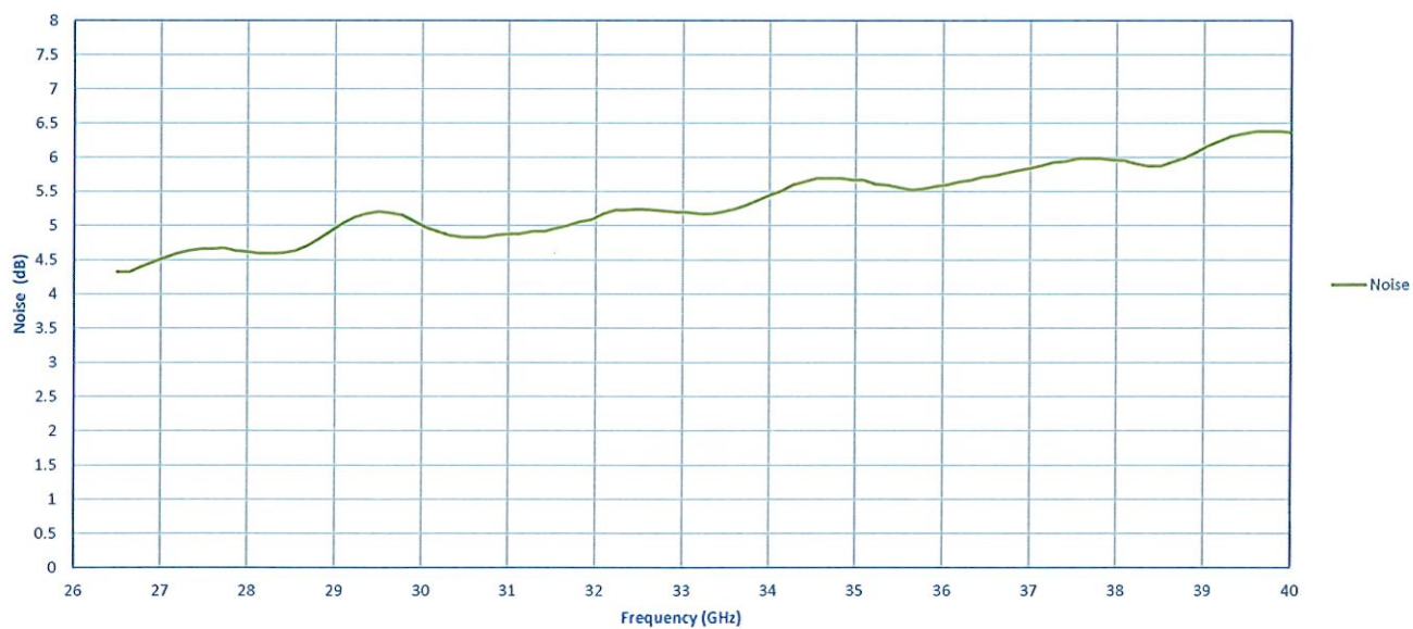
Noise Figure(26.5 to 40 GHz)
