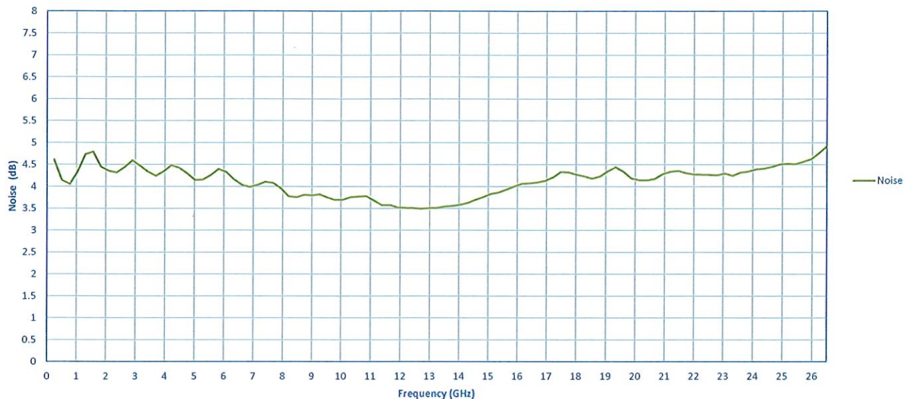
Noise Figure(0.25 to 26.5 GHz)
