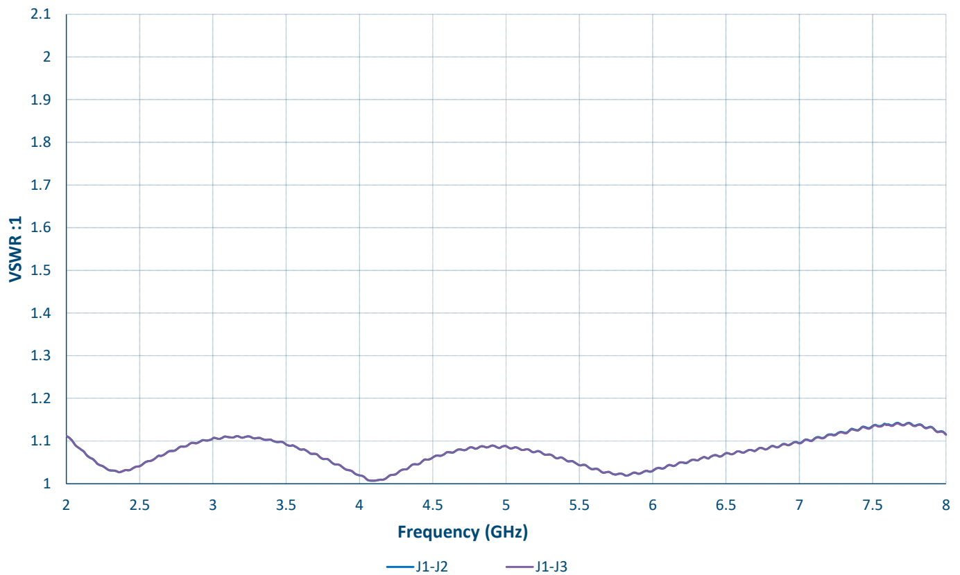
VSWR (J1)
