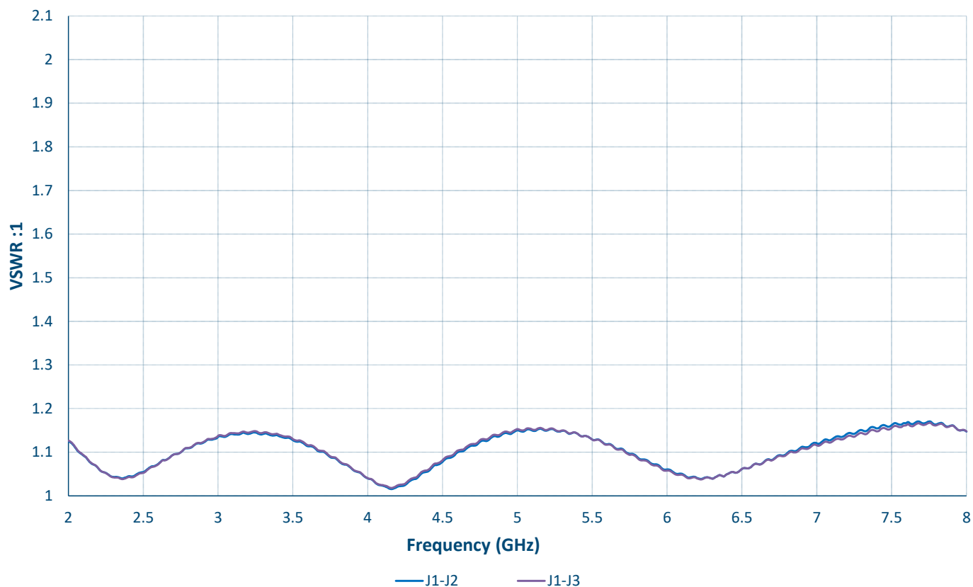
VSWR (J1)
