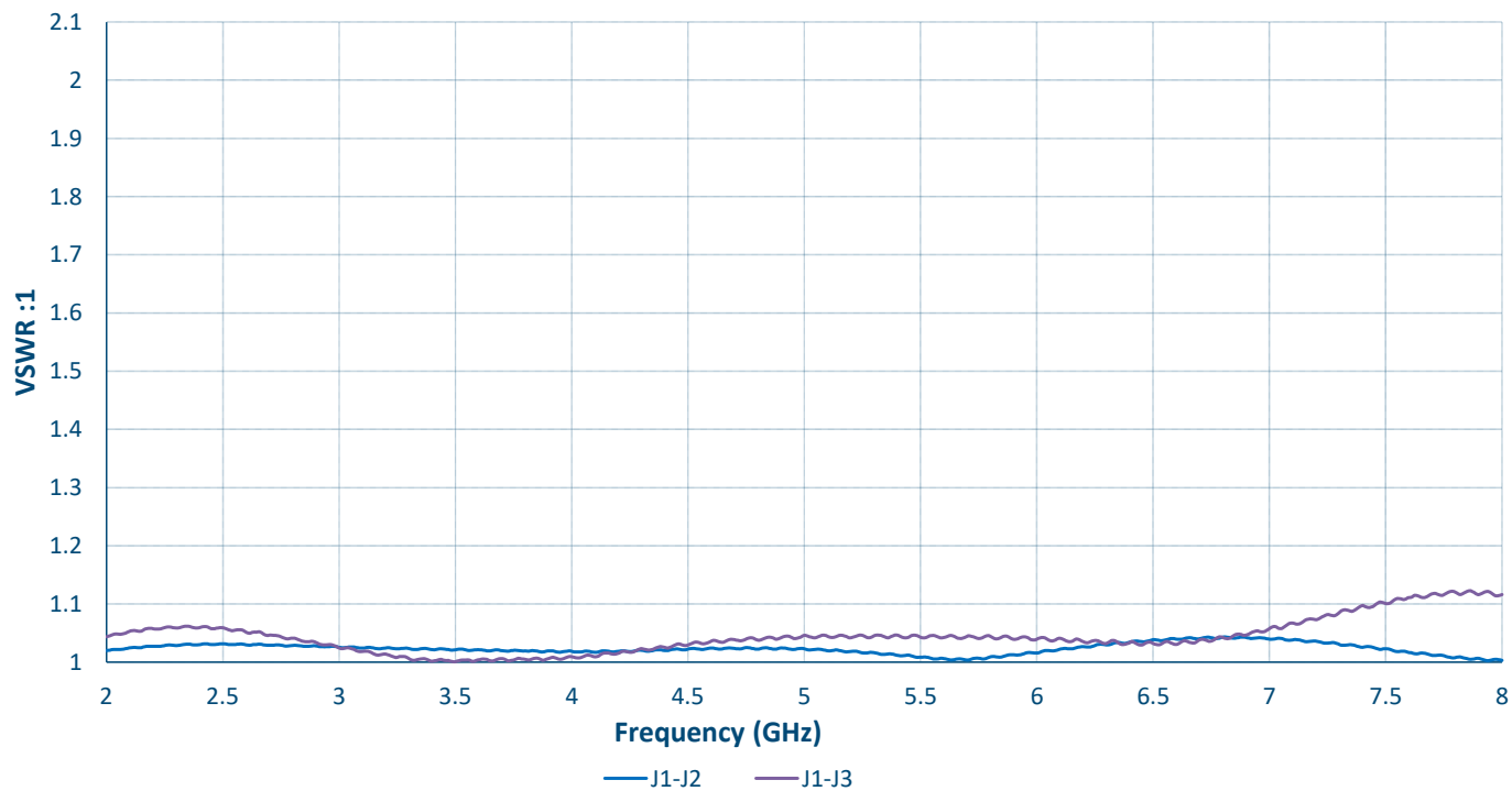
VSWR (J2, J3)
