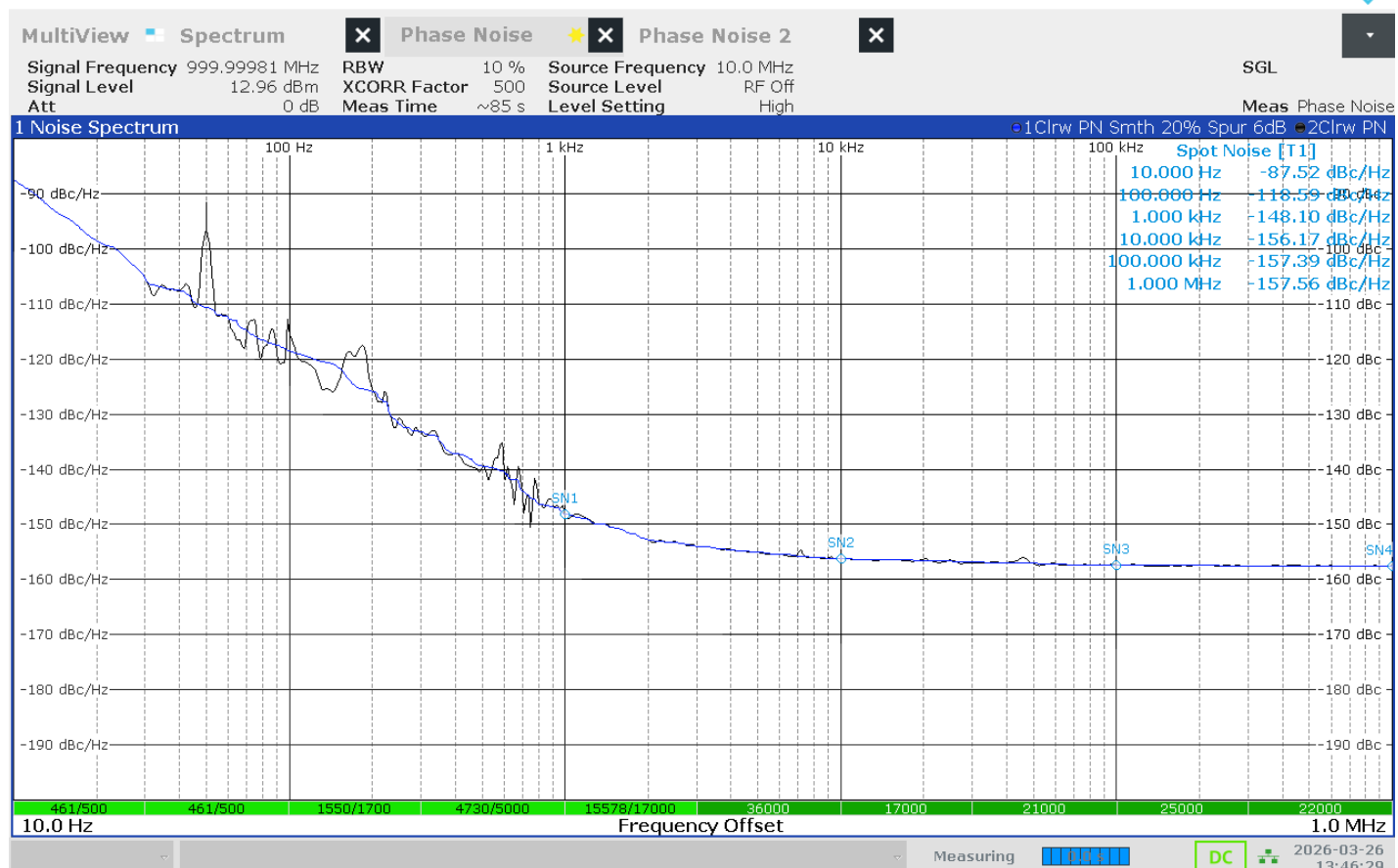
Figure 1: Typical Phase Noise @ 25°C
