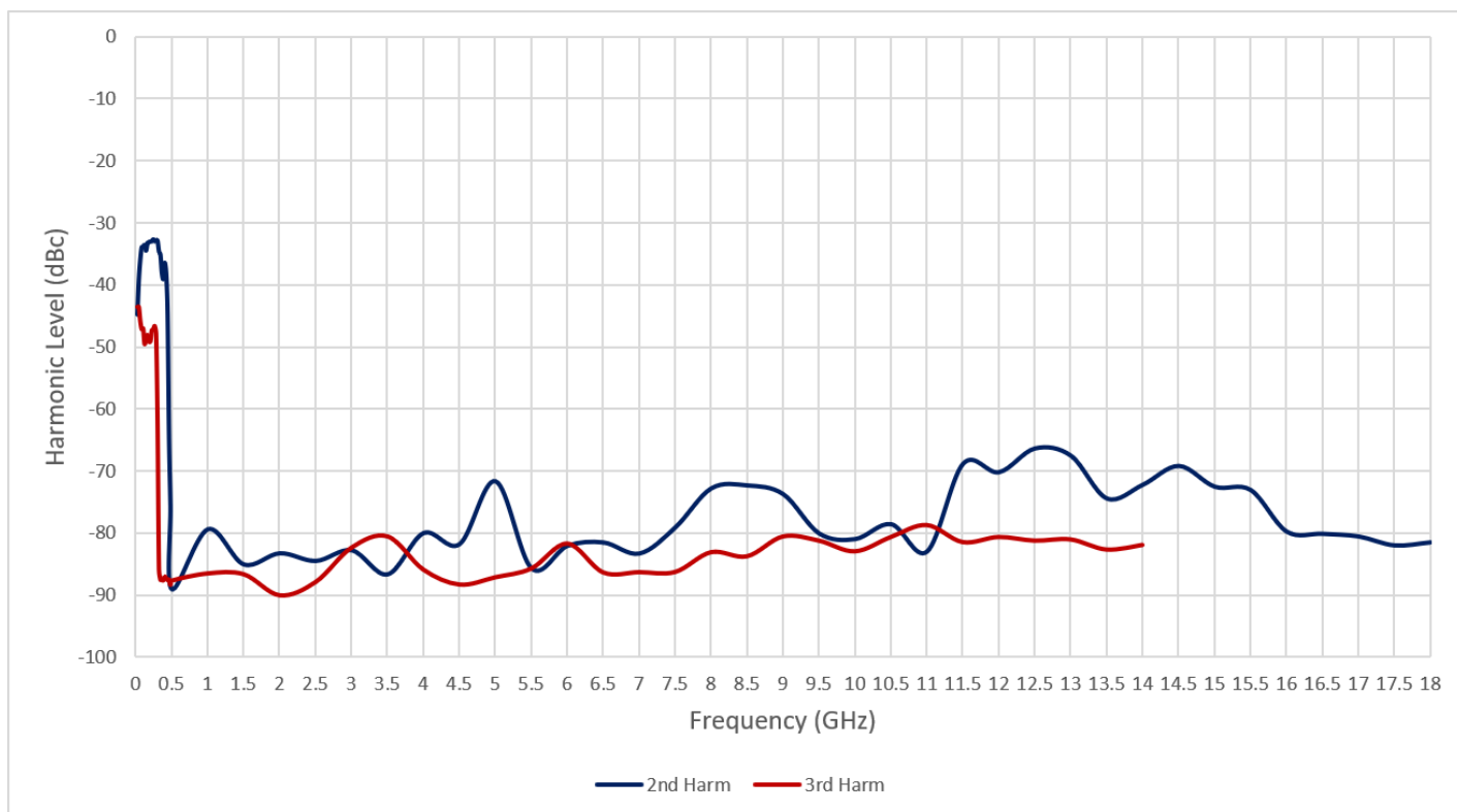
Figure 1: Measured Harmonic Levels @ 15 dBm Output Power
