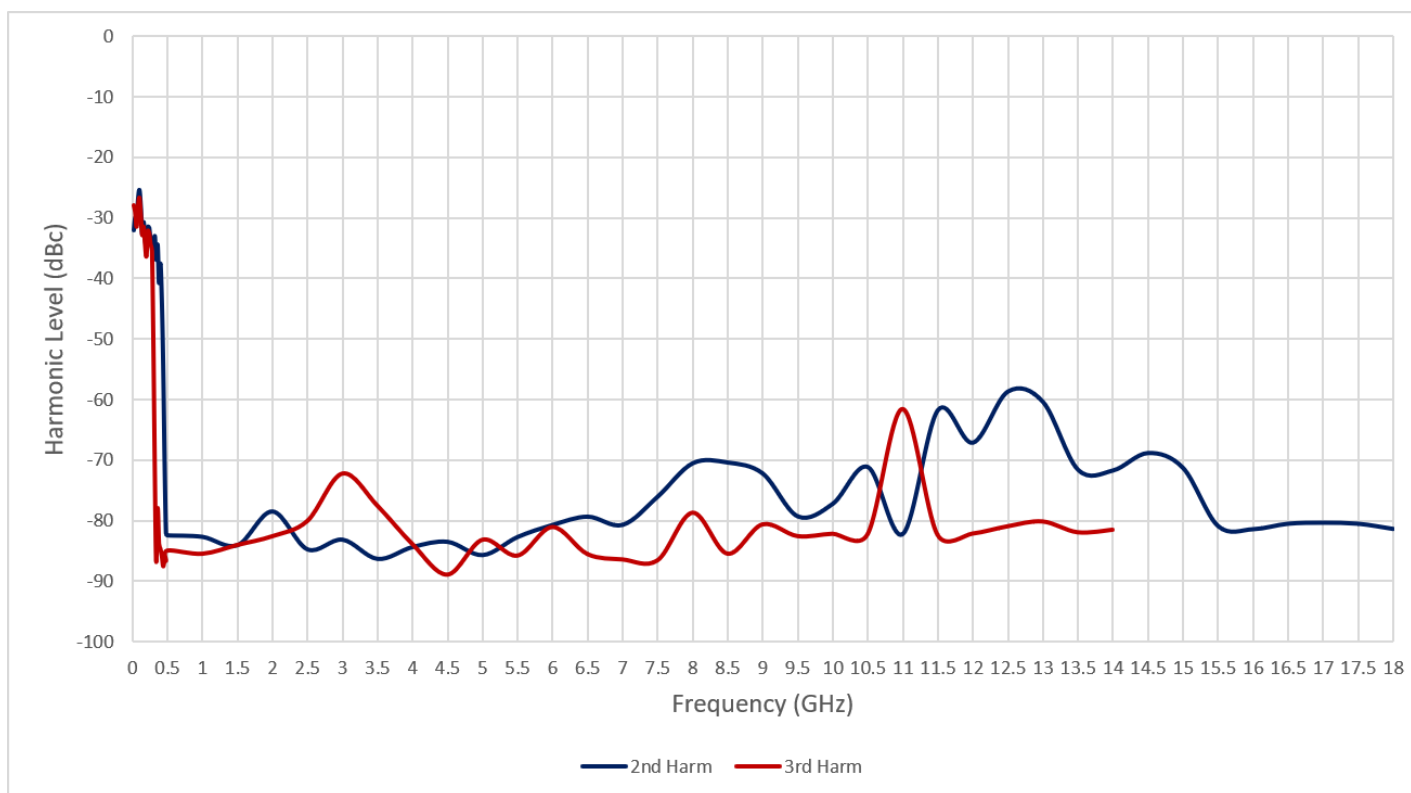
Figure 2: Measured Harmonic Levels @ 20 dBm Output Power
