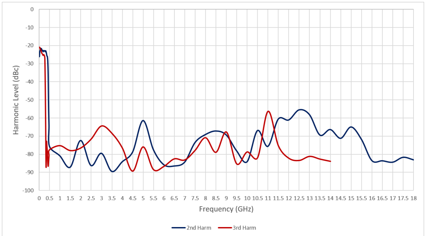
Figure 3: Measurement Harmonic Levels @ 23 dBm Output Power
