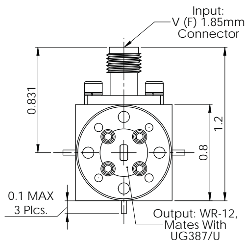
OUTLINE: Dimensions in inches (Not to scale)
