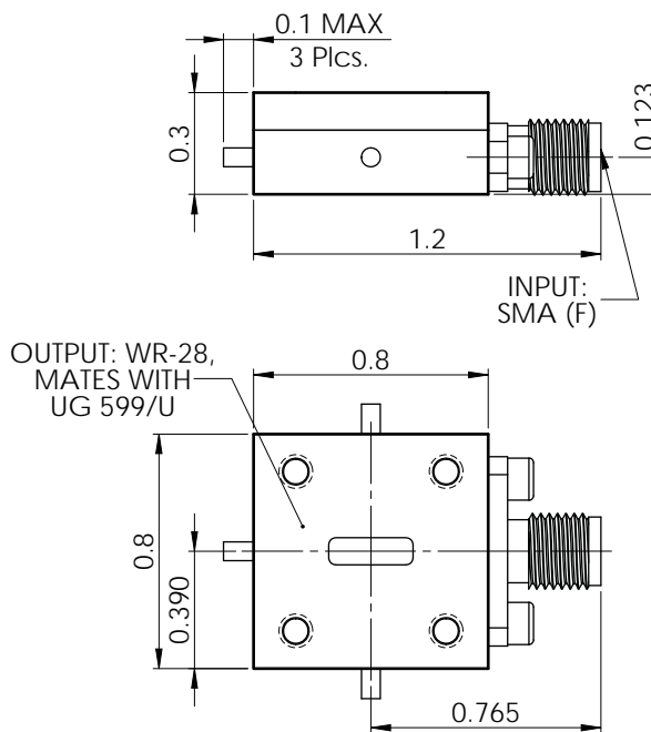
OUTLINE: Dimensions in inches (Not to scale)
