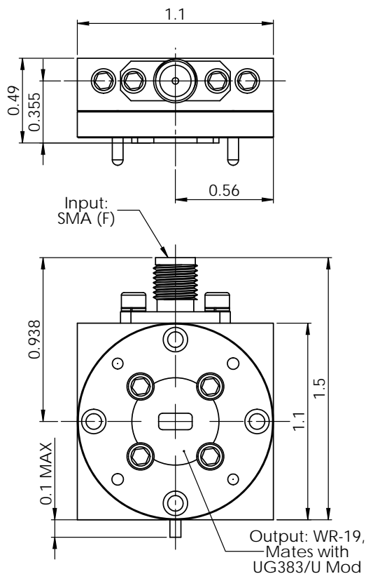
OUTLINE: Dimensions in inches (Not to scale)
