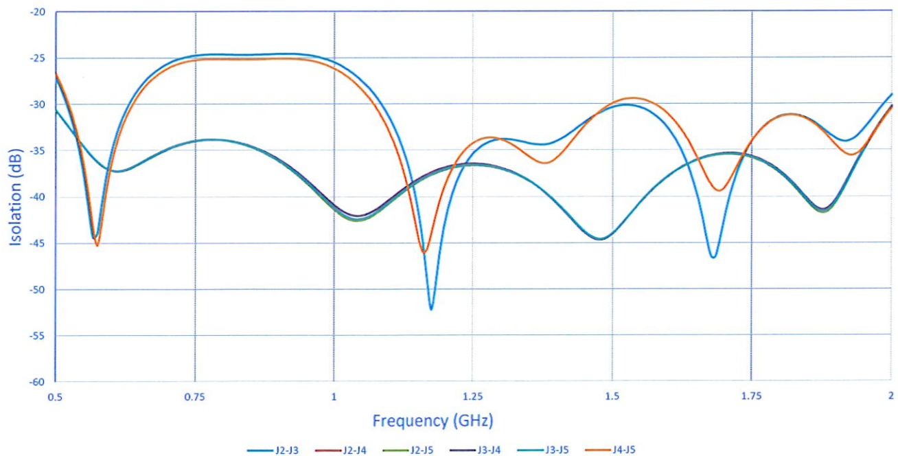
Isolation
