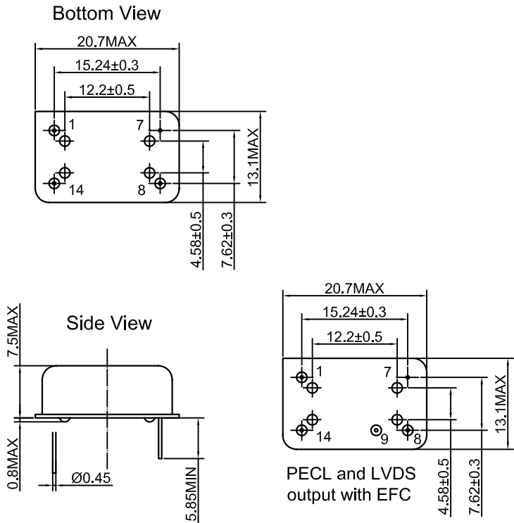
Pin Connections: (Without EFC)
