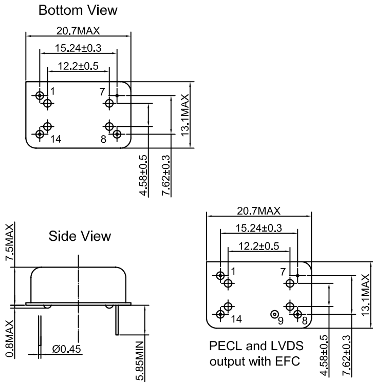
Pin Connections: (Without EFC)
