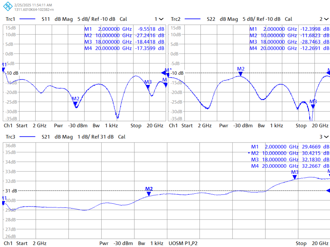
Figure 1: Small Signal Gain @ 25°C
