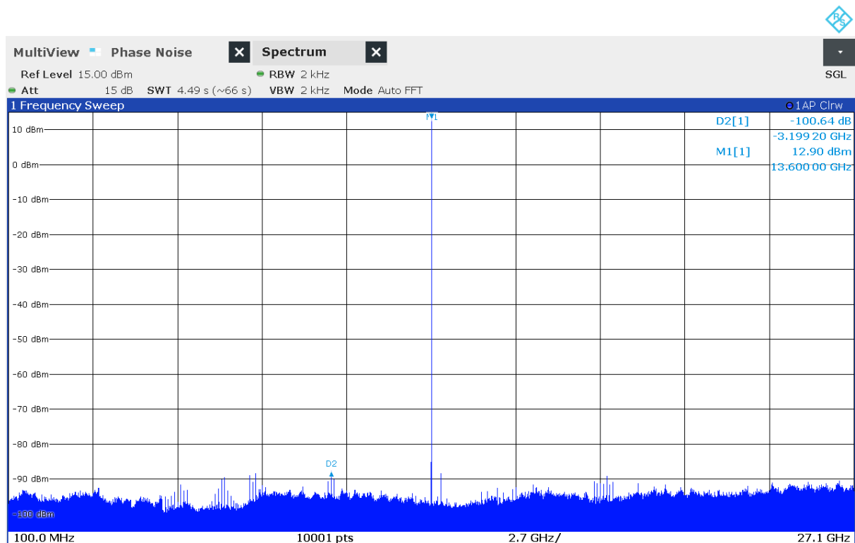
Figure 2: Spurious
