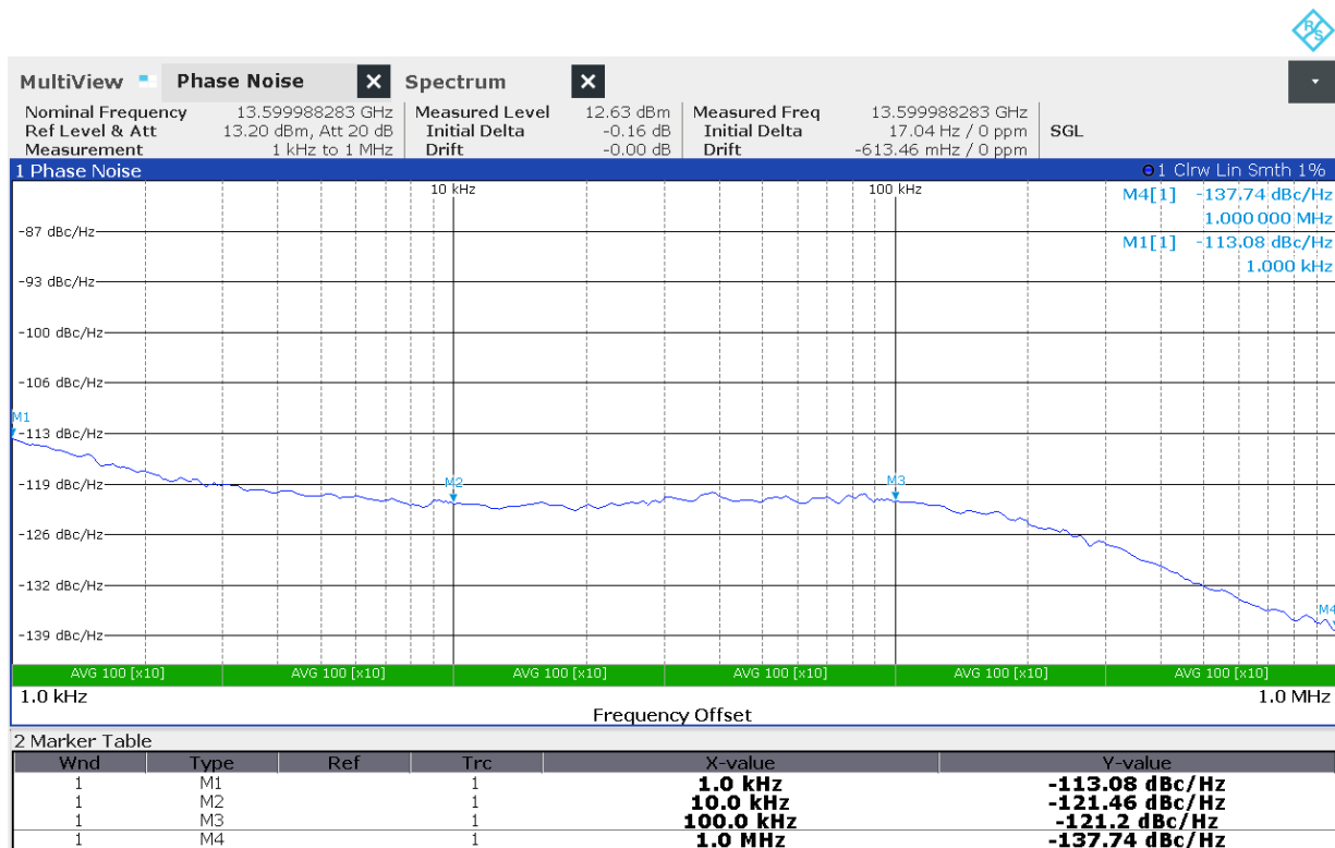
Figure 1: Phase Noise
