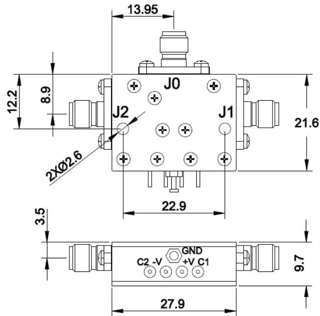
Figure 1: Mechanical Outline
