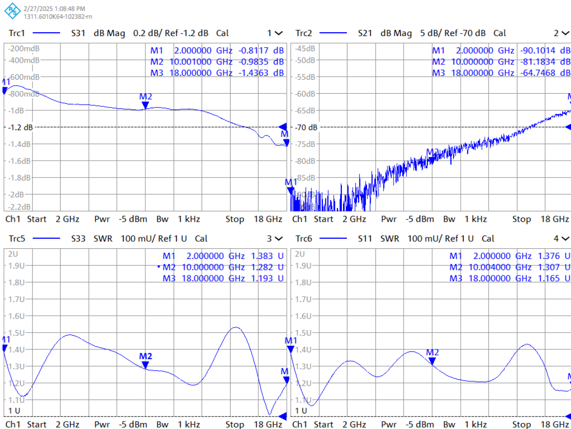
Figure 2: Typical Performance (Port1: J0, Port2: J1, Port3: J2)
