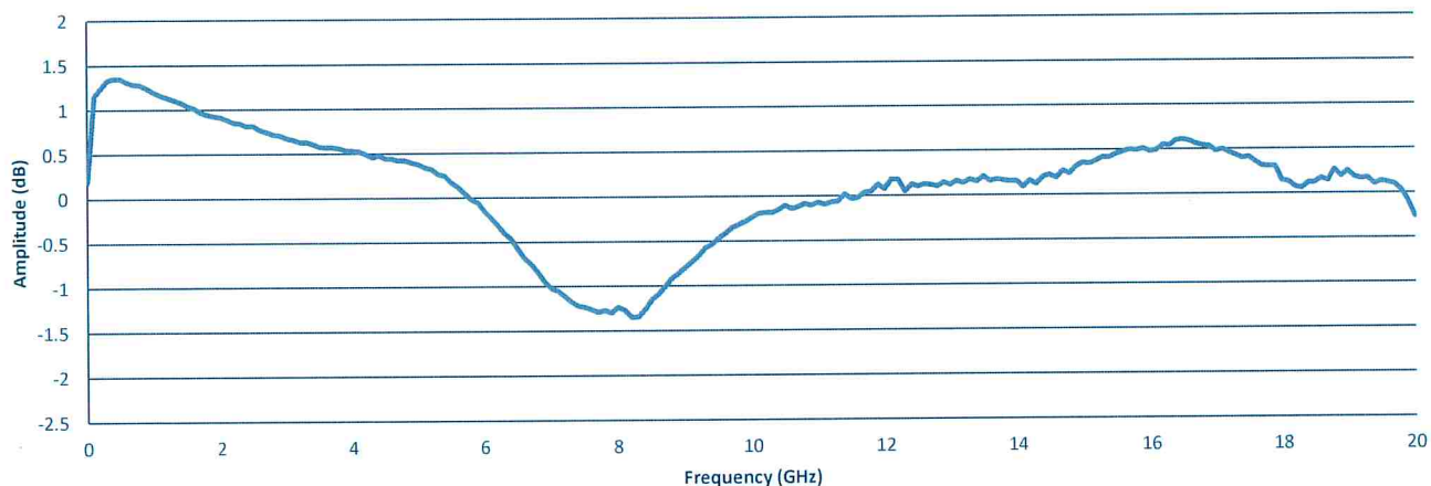
Gain Flatness
