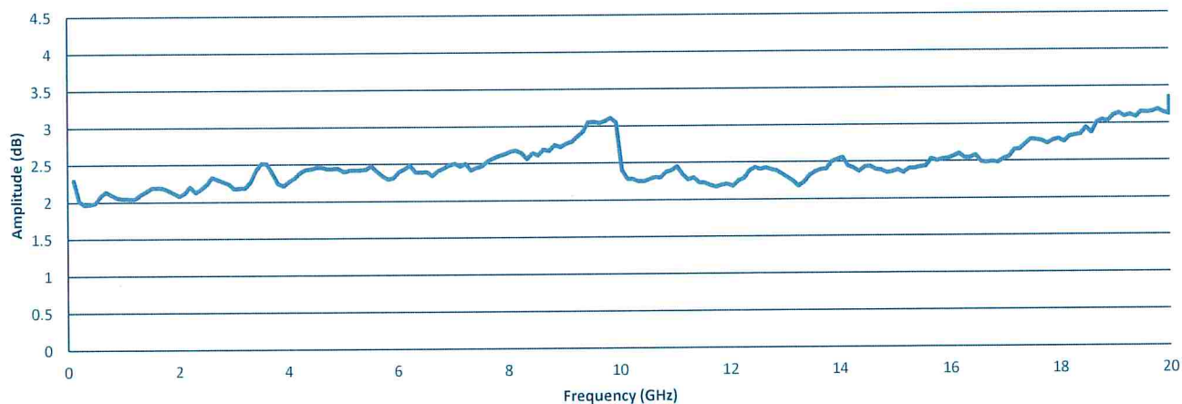
Noise Figure
