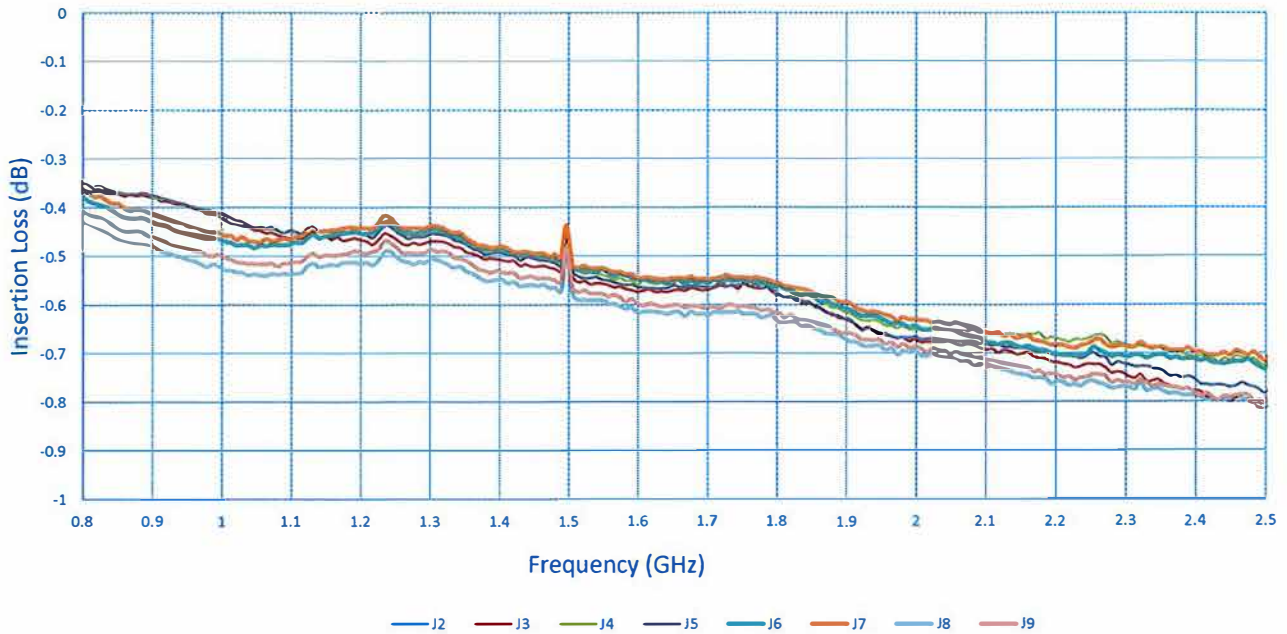
Insertion Loss
