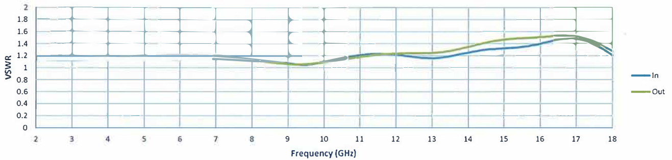
VSWR @ -10 dB
