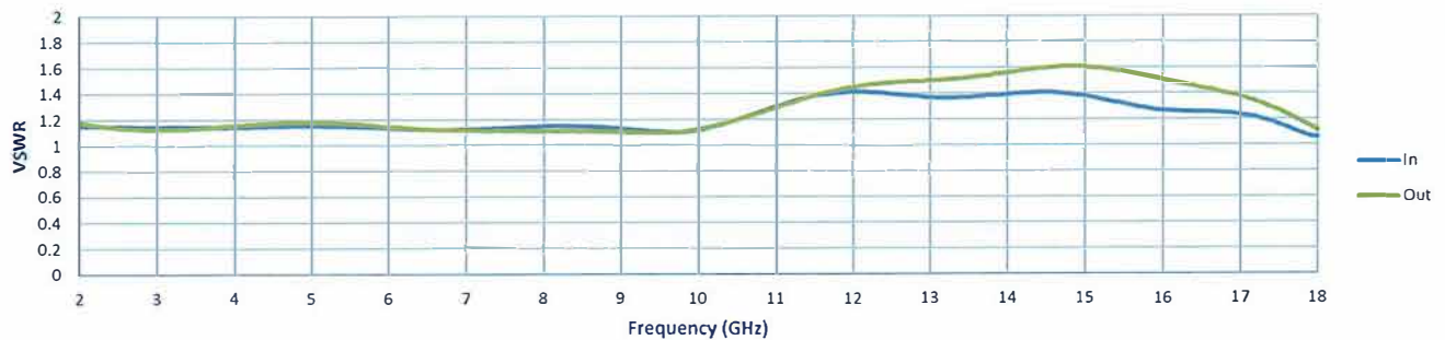
VSWR @ -10 dB
