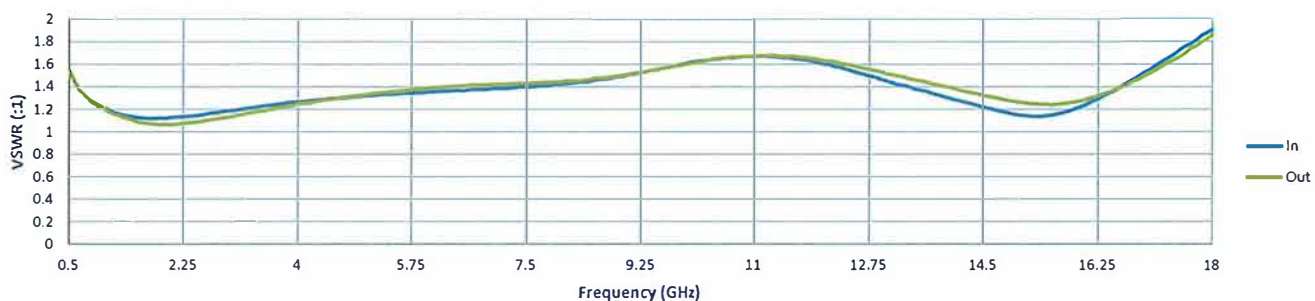
VSWR @ -20 dB
