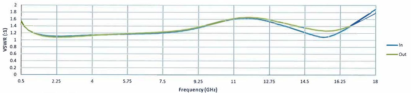
VSWR @ -20 dB
