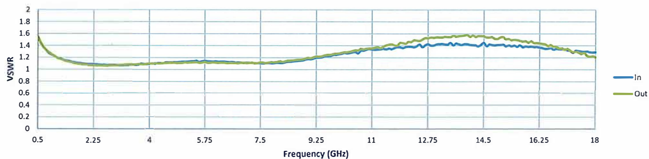
VSWR @ -20 dB
