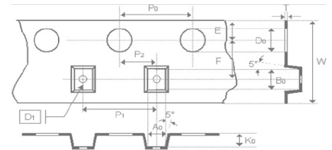
Plastic Tape Dimensions
