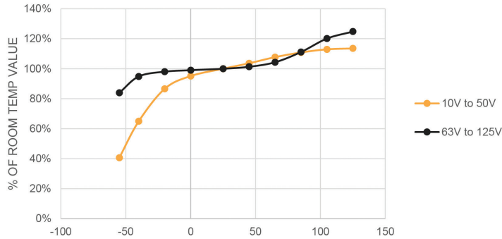
Typical Capacitance vs Temperature 120 Hz
