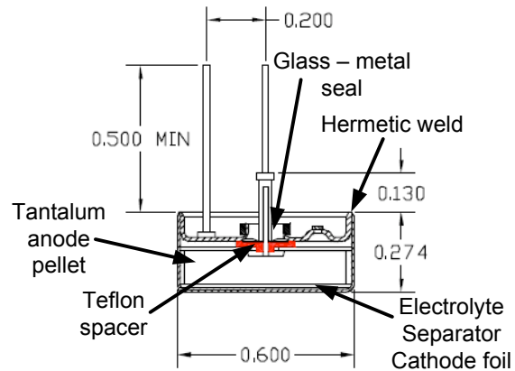
Fig. 1: Construction of the tantalum Hybrid capacitor THQA2016502.
