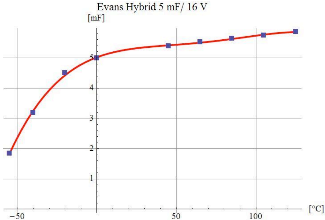
Fig. 8: Plot of capacitance vs. temperature.
