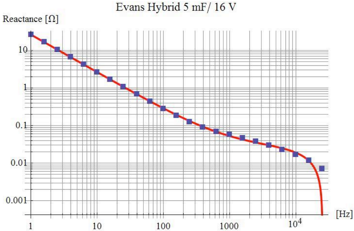
Fig. 5: Plot of reactance vs. frequency. The red line is an approximation by the function described below.
