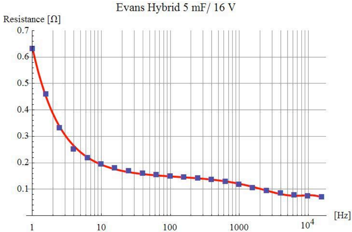
Fig. 4: Plot of ESR (resistance) vs. frequency and its approximation described below.
