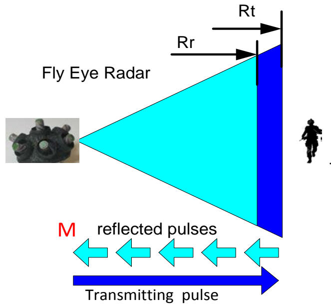
Figure 4. Range of detectable target R_r for Fly Eye radar.
