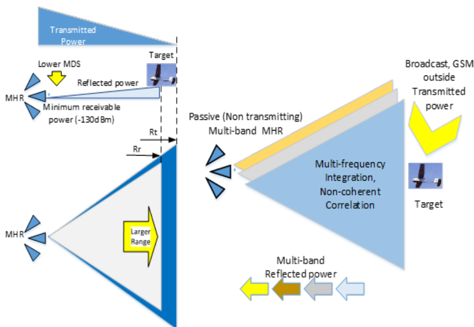
Figure 11. Passive radar concept. Multiband holographic radar (MHR) can use ambient energy sources.
