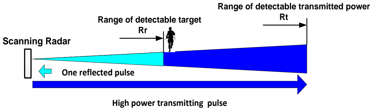
Figure 3. In regular scanning radar the range of detectable transmitted power R_t is larger for larger transmitting power and smaller beamwidth.
