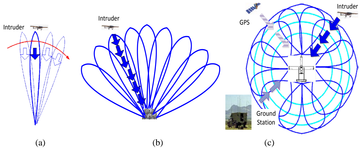
Figure 2. Scanning radar (a), monopulse radar (b) and Fly Eye radar (c).
