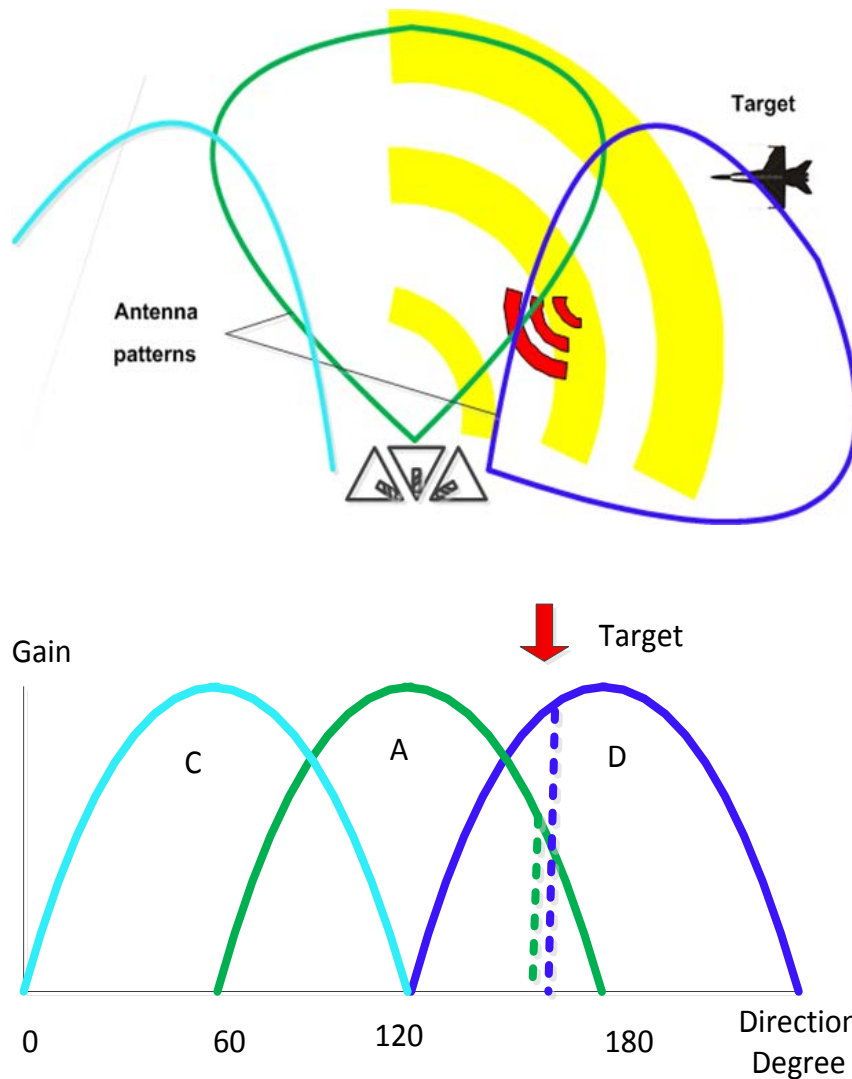
Figure 6. If the lobes of two antennas are overlapped, this signal can produce a high degree of pointing accuracy within the beam, adding to the natural accuracy of the conical scanning system.
