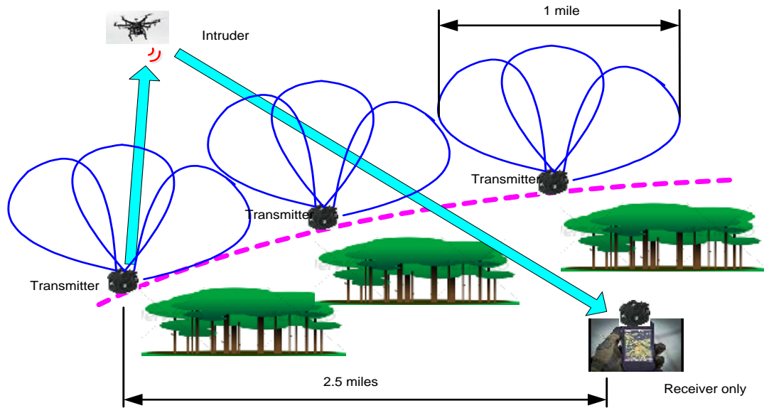
Figure 8. Transmitting modules can be distributed around perimeter of protected zone in bi-static drone detection system.
