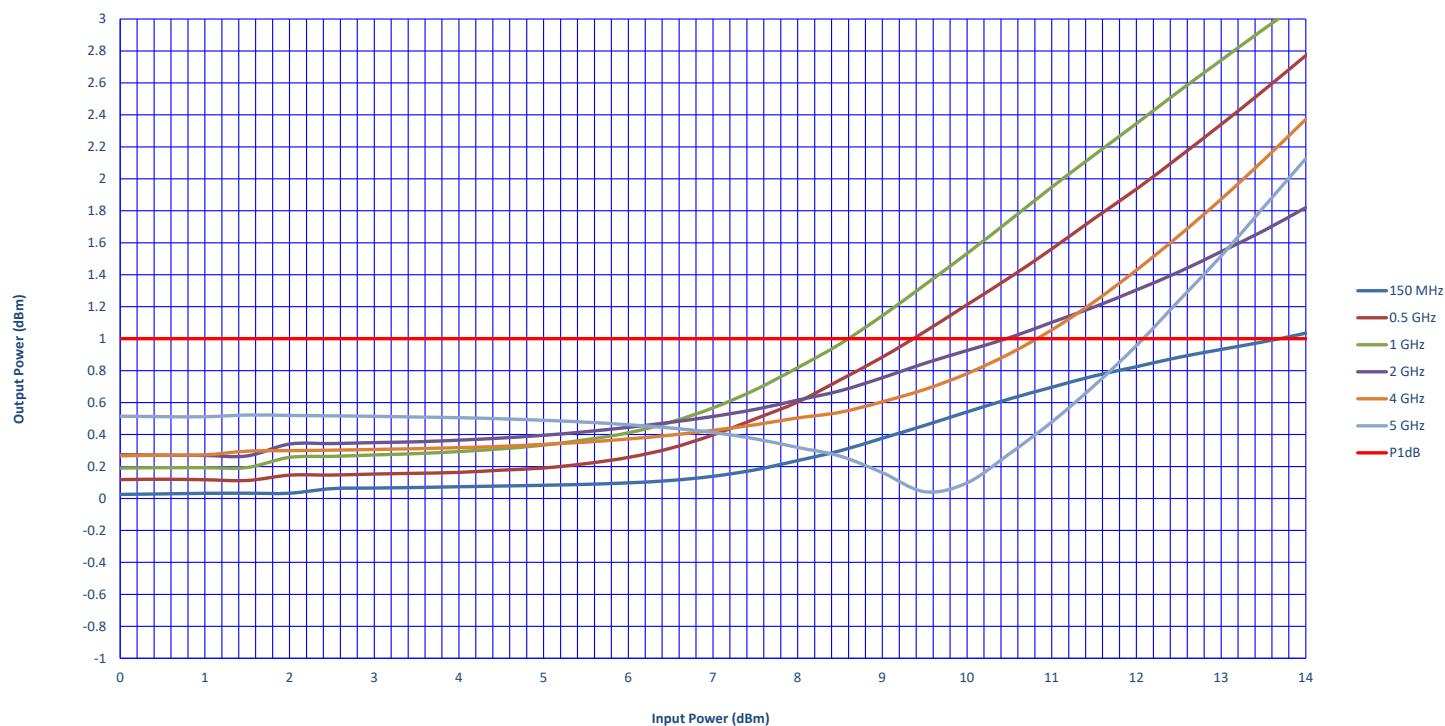
P1dB 150 MHz to 5 GHz @ (+25°C)
