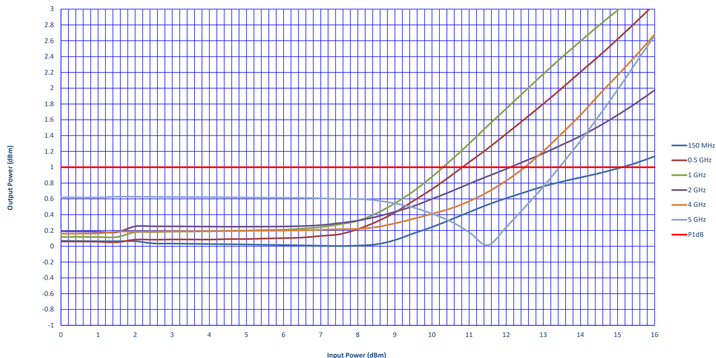
P1dB 150 MHz to 5 GHz @ (-55°C)
