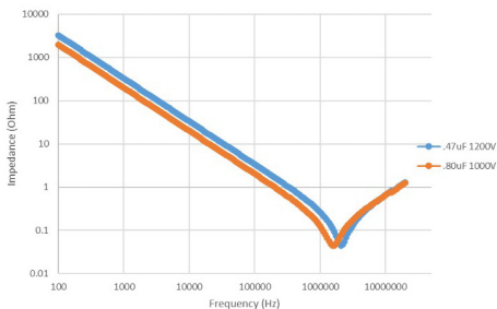
Impedance Vs Frequency
