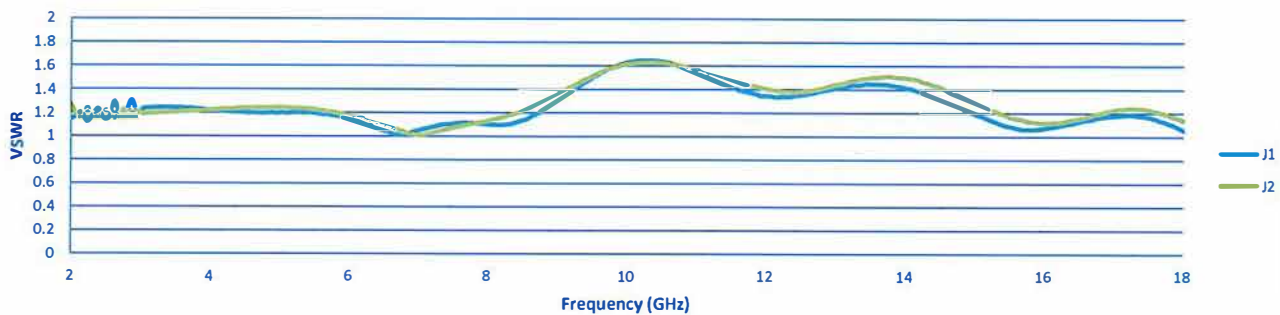
VSWR @ -10 dB
