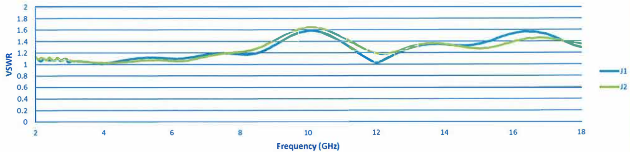
VSWR @ -10 dB
