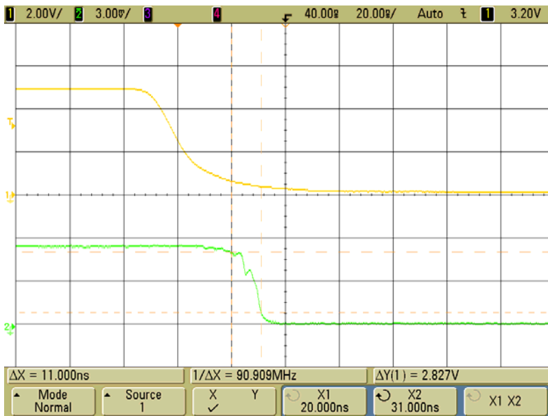
Yellow Trace TTL Input Signal Green Trace RF Output of Detector
