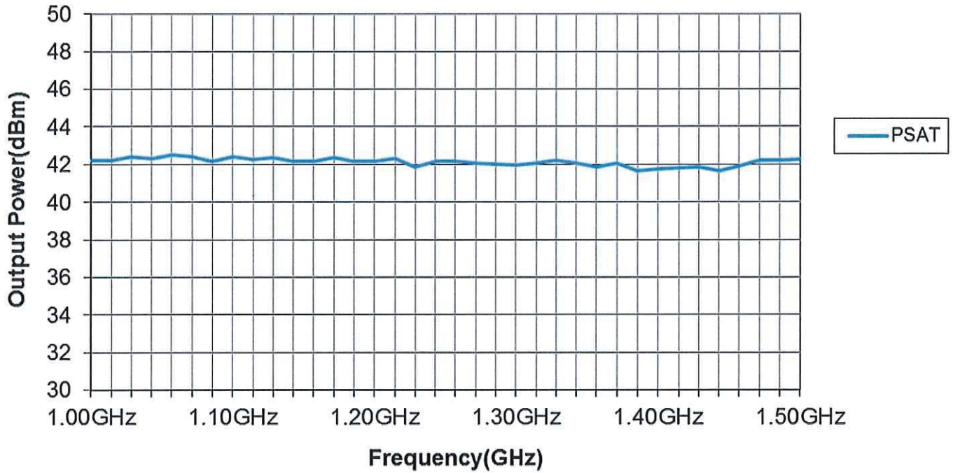
Saturated Output Power vs Frequency @+25C
