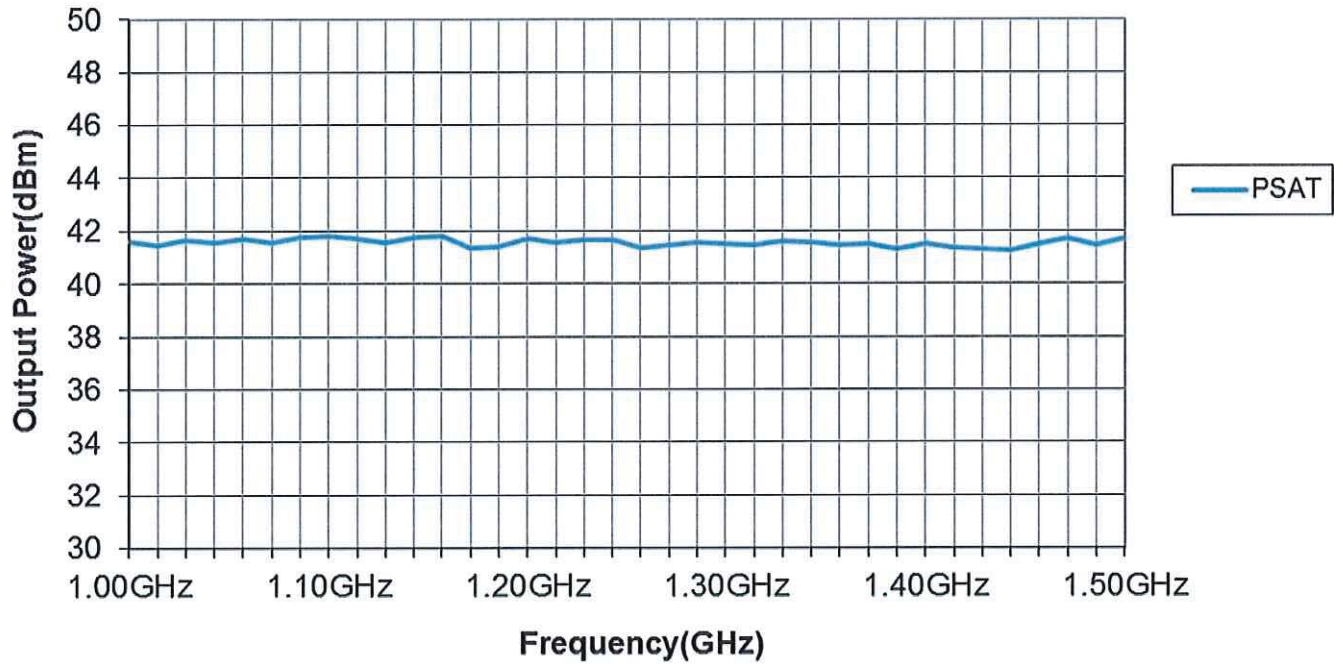
Saturated Output Power vs Frequency @+85C
