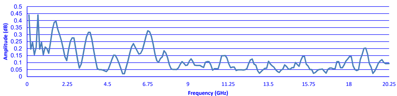
Gain Flatness any 500 MHz Span
