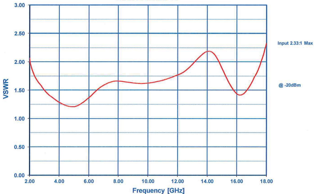
VSWR GRAPH
