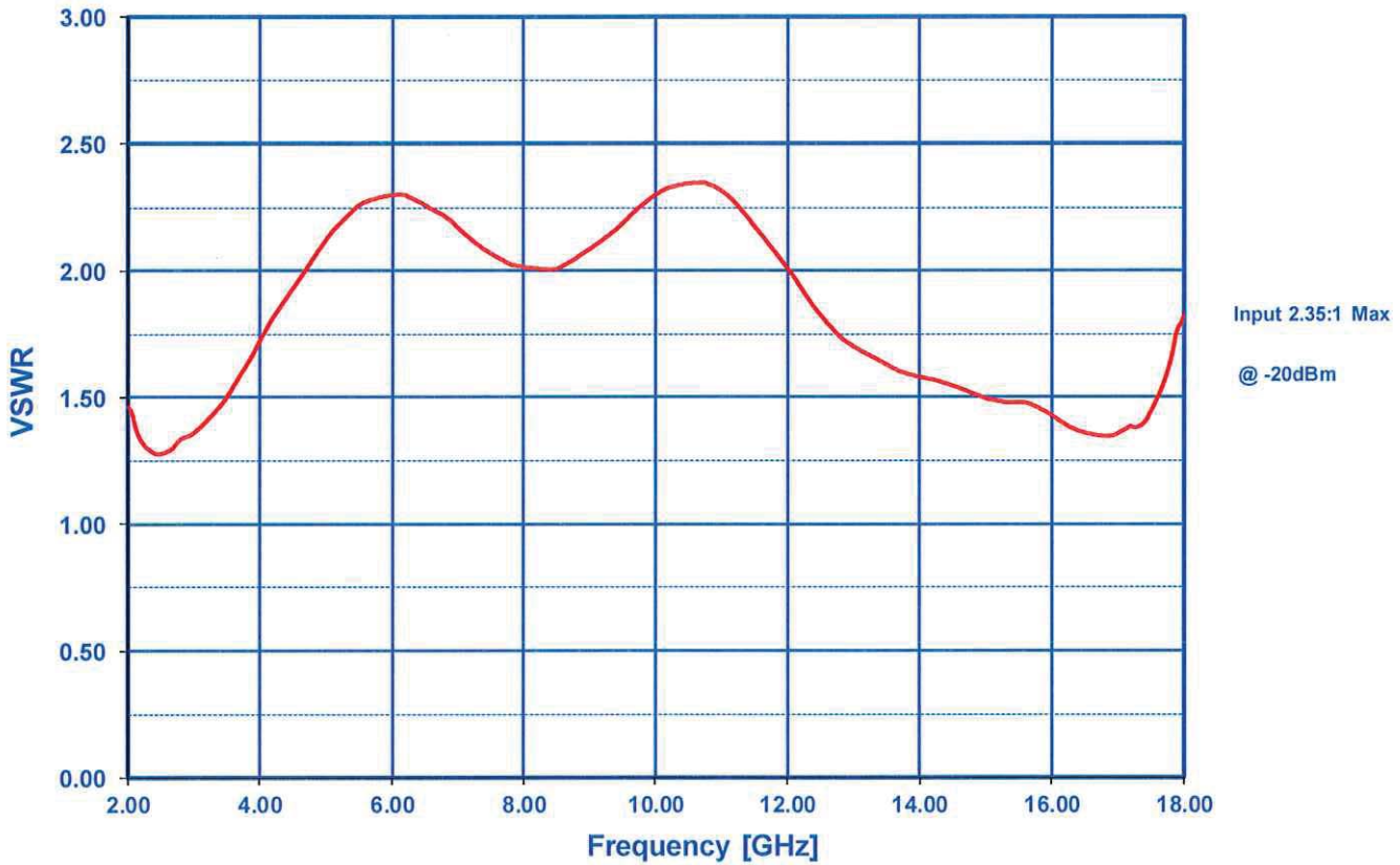
VSWR GRAPH
