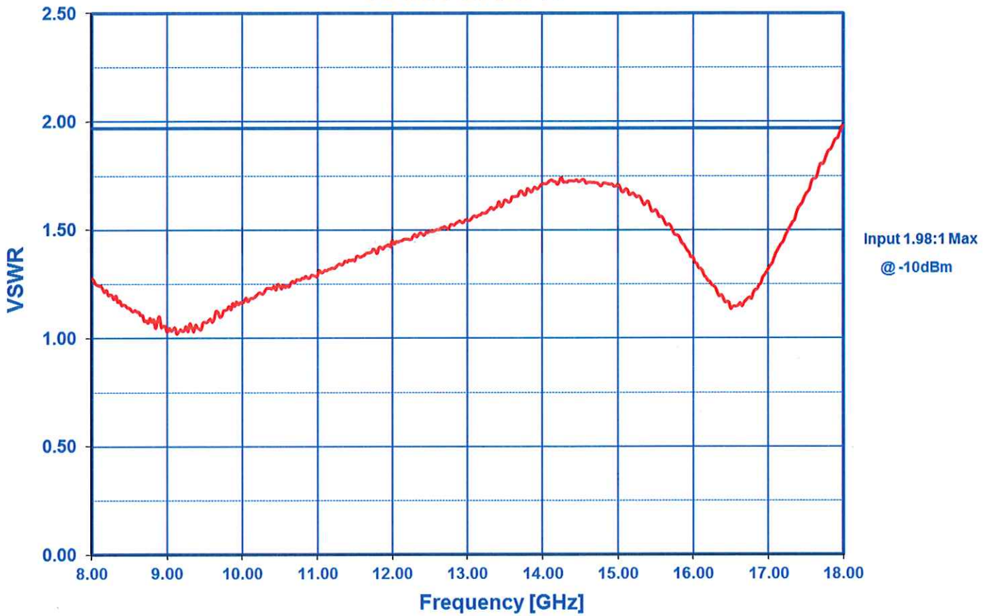
VSWR GRAPH
