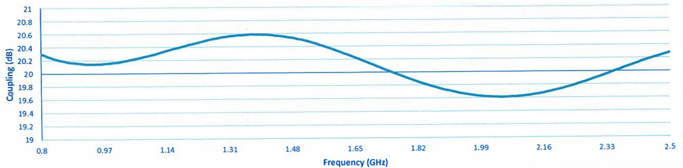
Coupling
