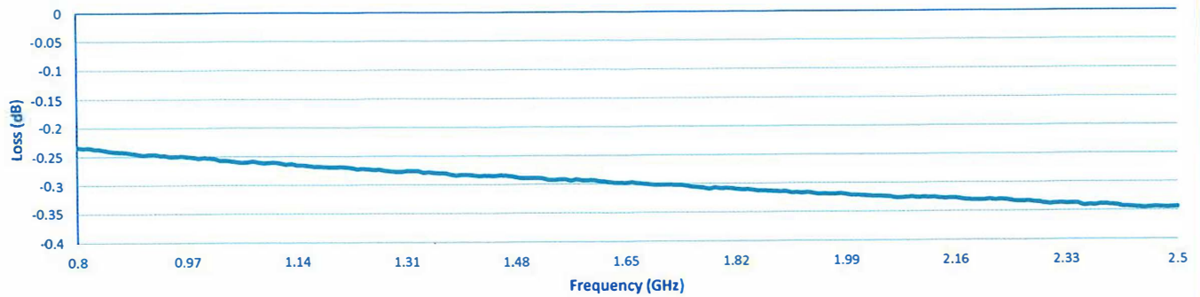
Insertion Loss
