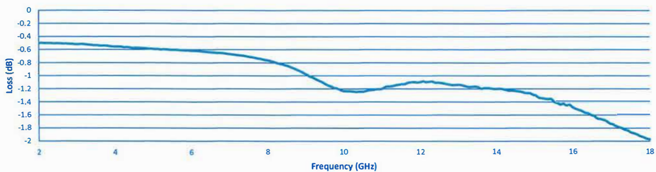
Insertion Loss @ -10 dB
