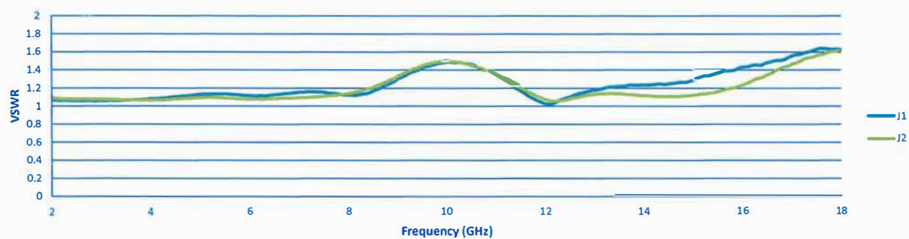
VSWR @ -10 dB
