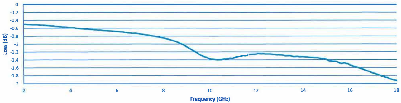
Insertion Loss @ -10 dB
