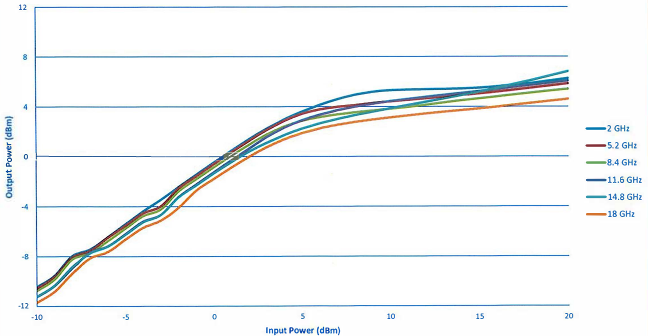
Limiter Response with Frequency
