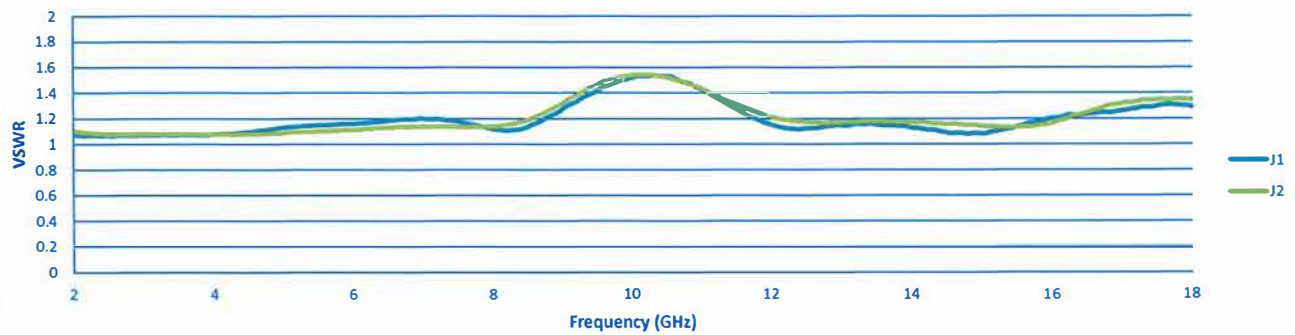
VSWR @ -10 dB
