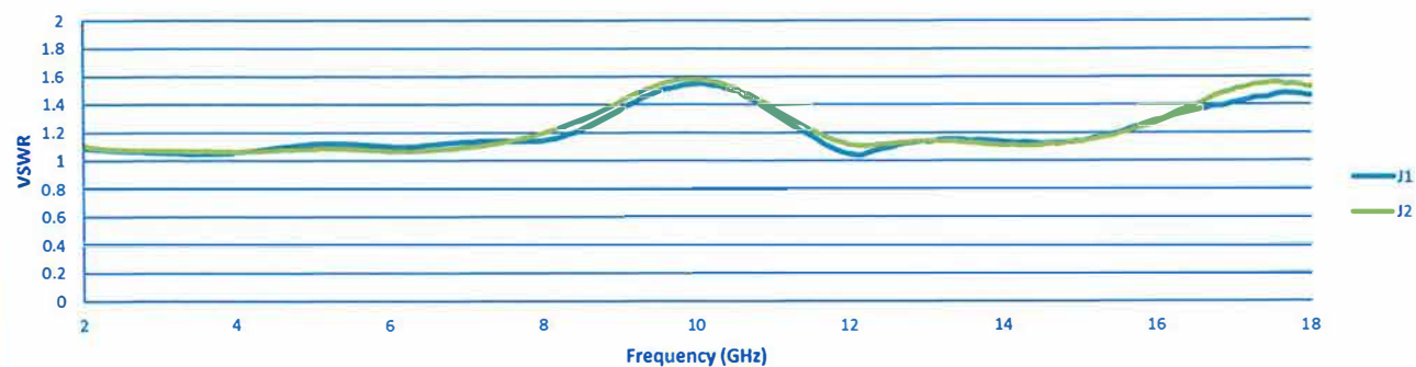
VSWR @ -10 dB
