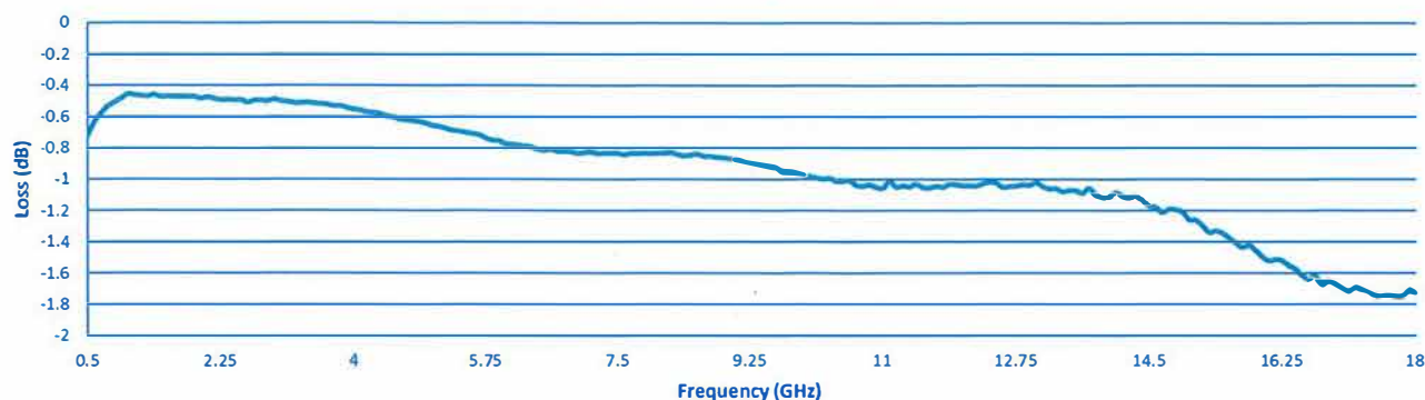
Insertion Loss @ -20 dB
