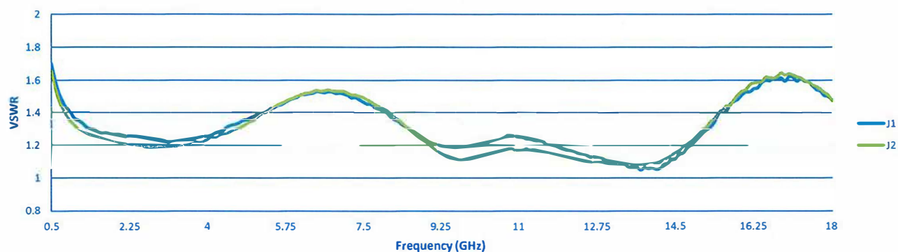
VSWR @ -20 dB
