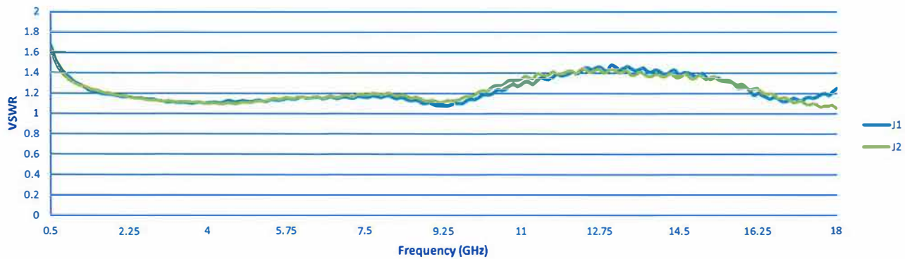
VSWR @ -20 dB
