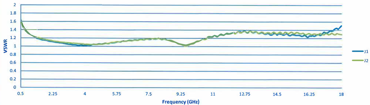
VSWR @ -20 dB
